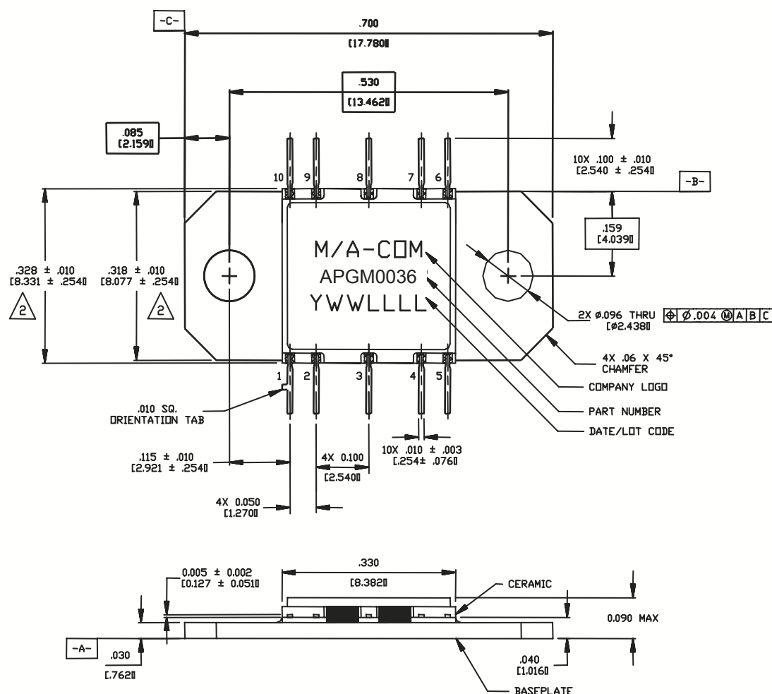
Figure 5. CR-15 Package Dimensions
