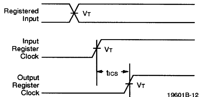
Input Register to Output Register Setup (MACH 2 and 4)
