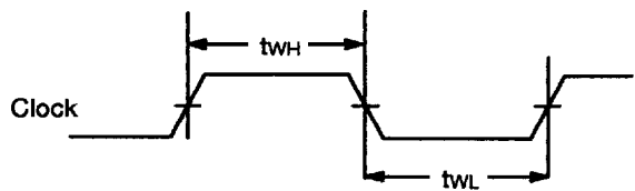
Clock Width
