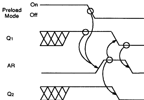
Figure 1. Preload/Reset Conflict
