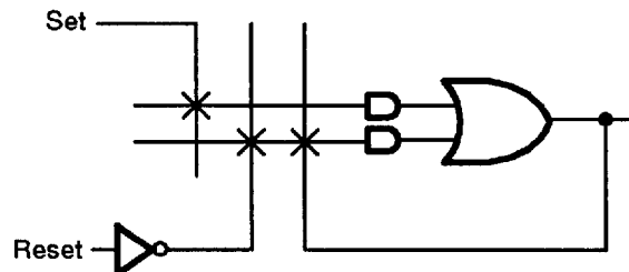
Figure 2. Combinatorial Latch
