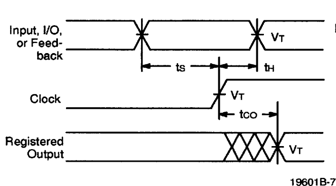
Registered Output
