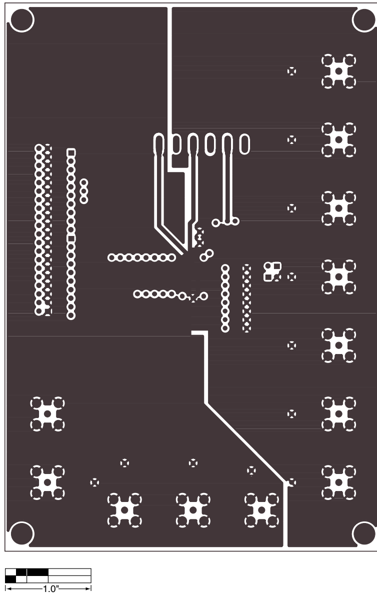
Figure 5. MAX1294 EV Kit PC Board Layout—Interior Layer 2
