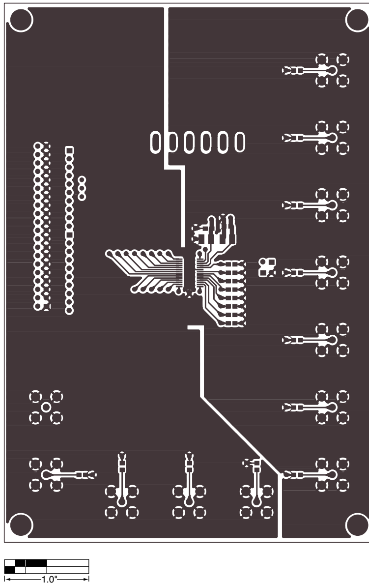
Figure 3. MAX1294 EV Kit PC Board Layout—Component Side
