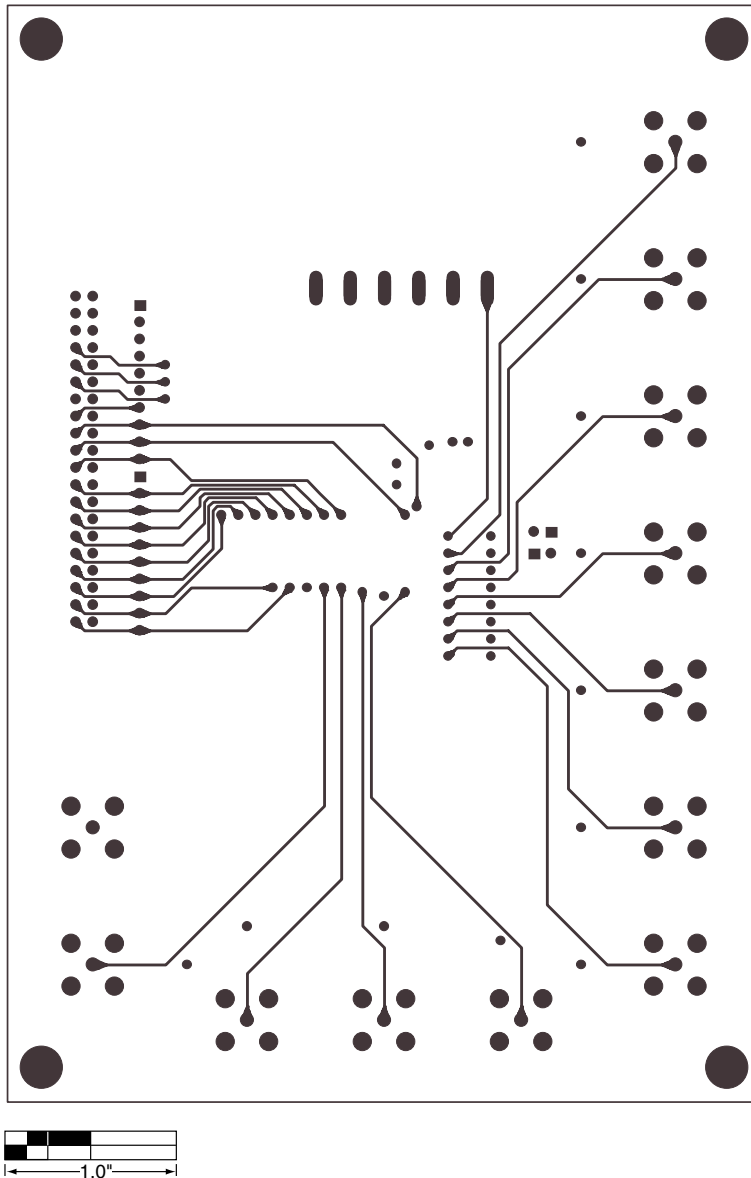
Figure 6. MAX1294 EV Kit PC Board Layout—Solder Side
