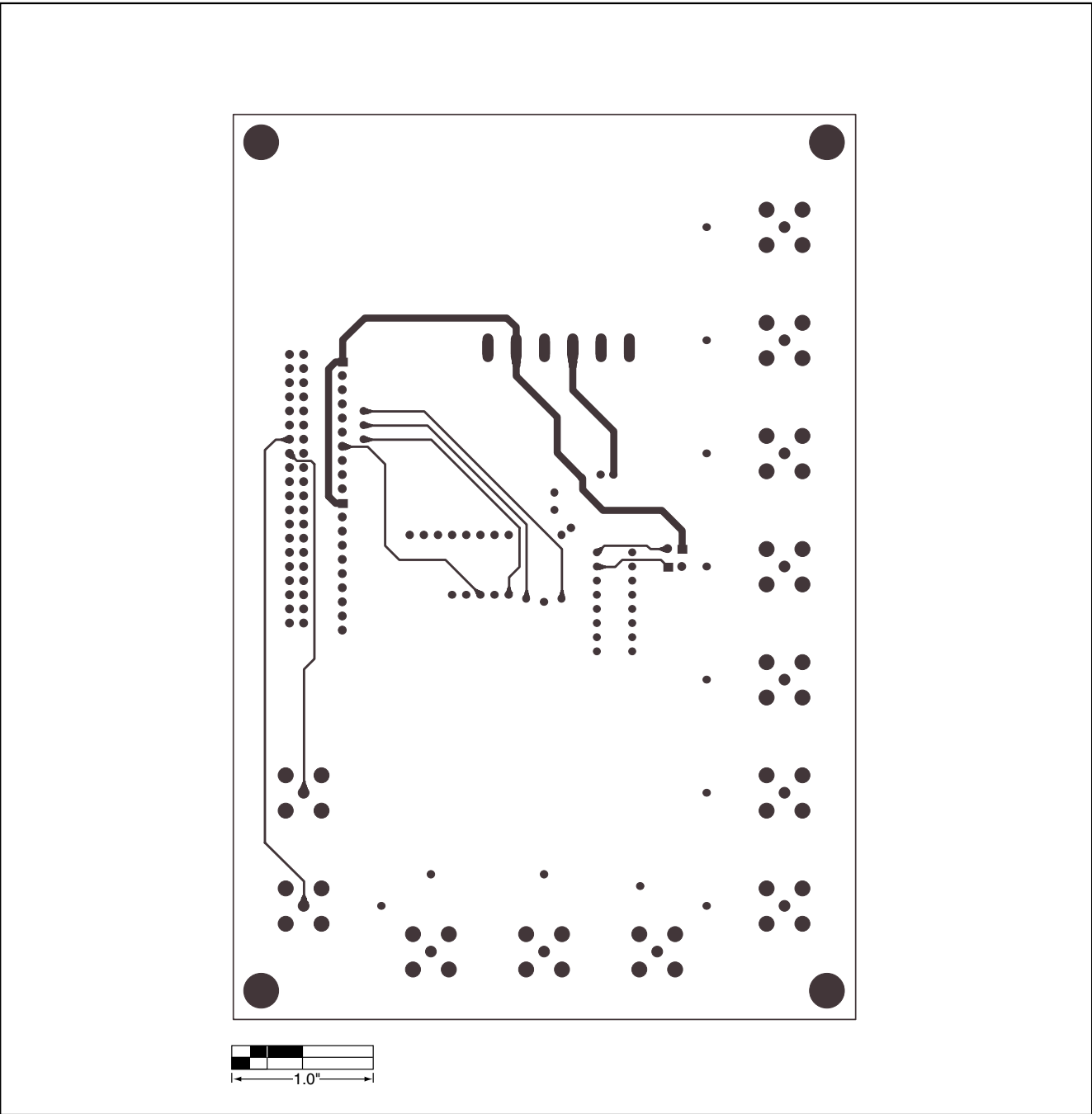
Figure 4. MAX1294 EV Kit PC Board Layout—Interior Layer 1
