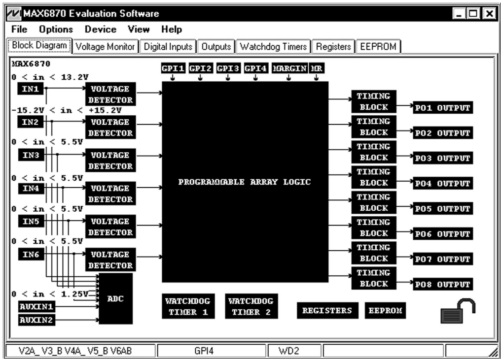
Figure 1. Block Diagram (Can Be Brought Up Anytime by Pressing Function Key F1)
