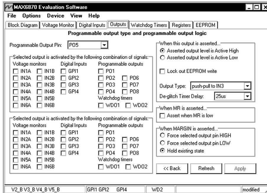
Figure 5. Programmable Outputs
