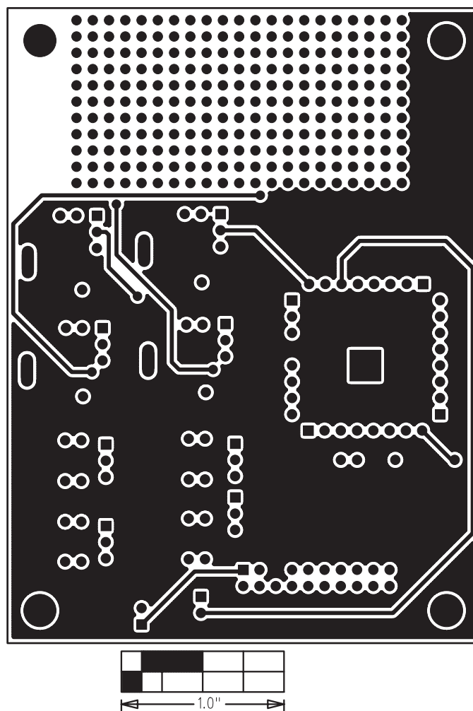
Figure 12. MAX6870 EV Kit PC Board Layout—Solder Side
