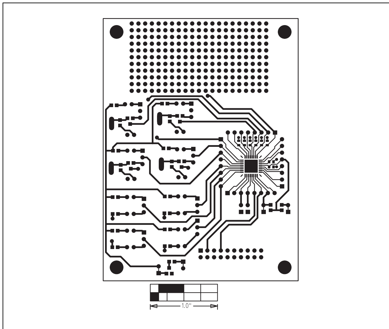
Figure 11. MAX6870 EV Kit PC Board Layout—Component Side
