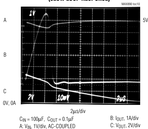
OUTPUT OVER-LOAD (SLOW LOOP RESPONSE)
