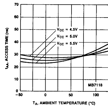
t_{AA} Access Time vs. Ambient Temperature
