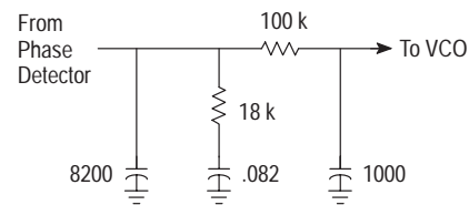
Figure 102. Open Loop Response Basaset US with Selected Values
