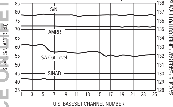
Figure 66. Typical Performance Parameters Over U.S. BaseSet Channel Frequencies
