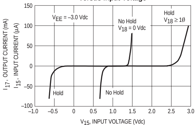
Figure 16. Data Slicer Input Current versus Input Voltage
