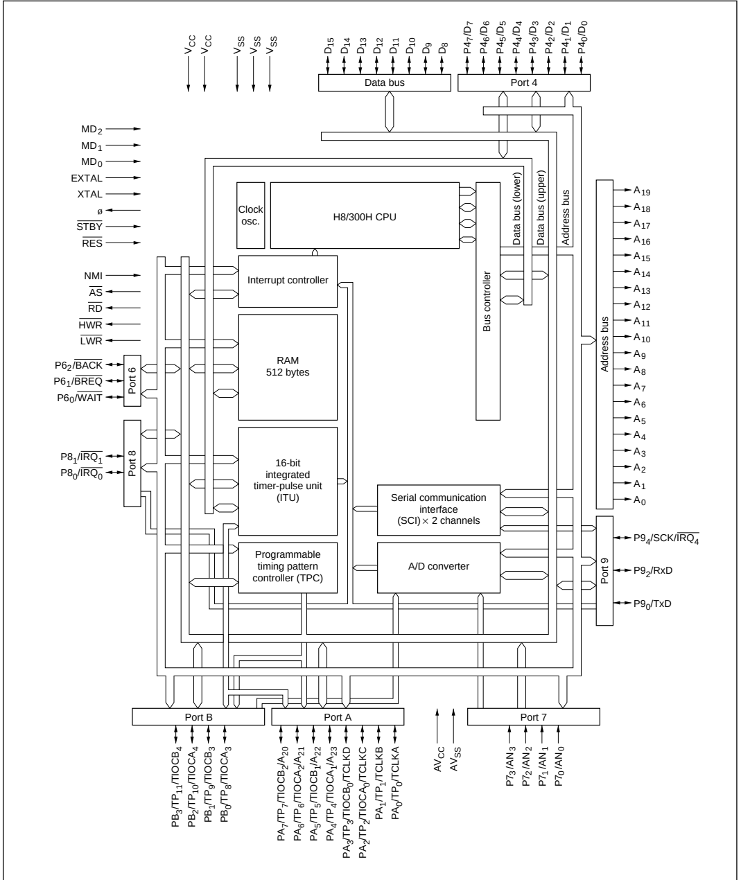
Figure 1-1 Block Diagram of H8/3001
