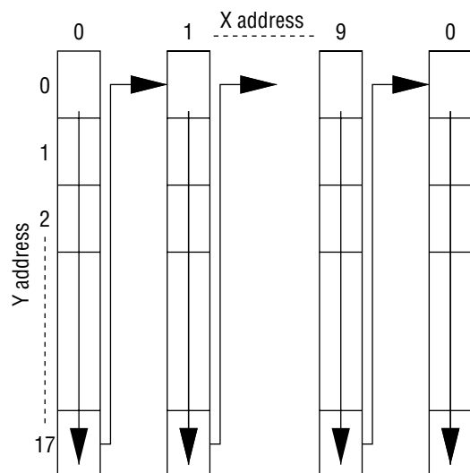
2. Y address increment example (8-bit word length, 1/18 duty)
