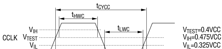
Figure 6.4 CardBus Clock Waveform
