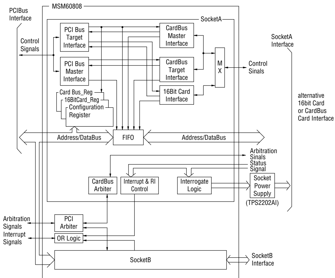
Figure 2. Block Diagram
