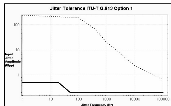
Figure 8 - Jitter Tolerance ITU-T G.813 Option 1
