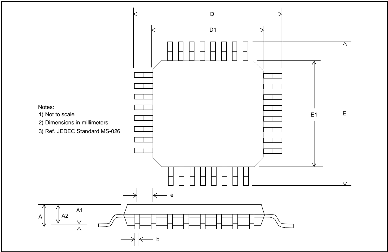
MT90401AB 80 Pin LQFP
