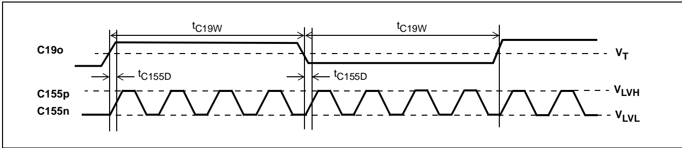
Figure 19 - Output Timing 2
