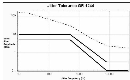
Figure 7 - Jitter Tolerance GR-1244 1.544MHz Reference
