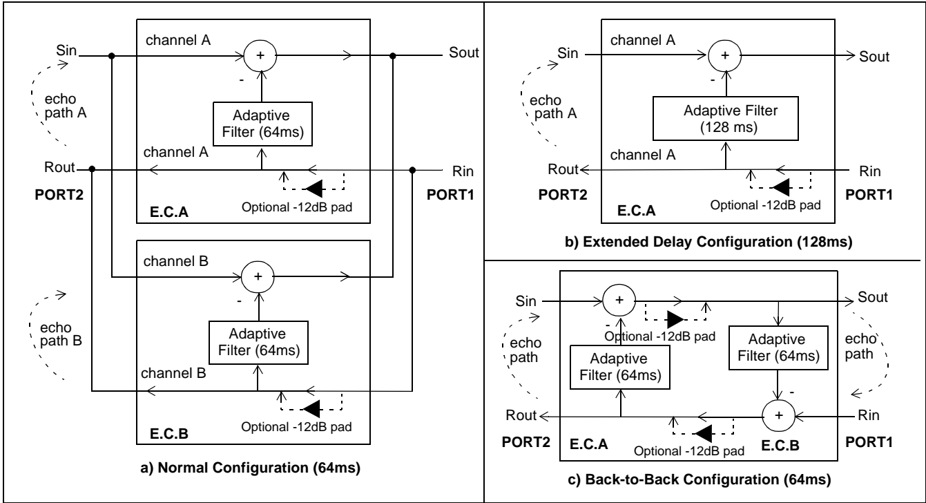
Figure 5 - Device configuration
