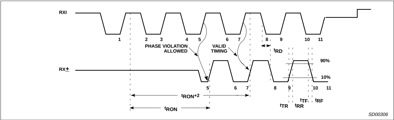
Figure 3. Receiver Timing
