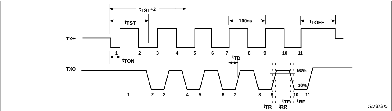
Figure 5. Transmitter Timing
