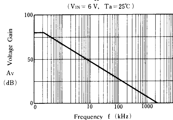
Voltage Gain
