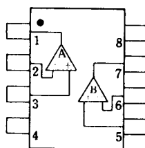
NJM353D NJM353M
