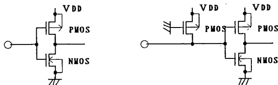
Input Terminal Structure
