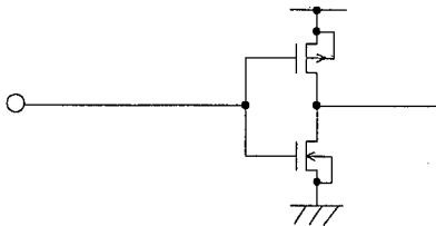
Input/Output Terminal Structure SIO Terminal
