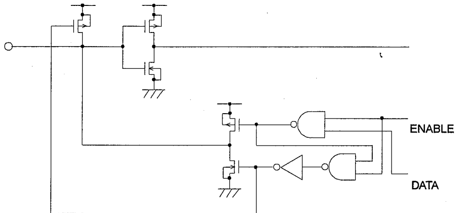
Input/Output Terminal Structure SIO Terminal
