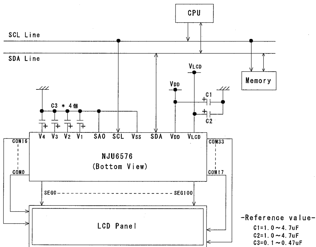
Fig.15 Typical application circuit
