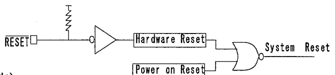
Fig.3 Reset circuit
