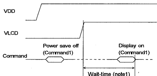
Fig.8 Power supply on timing and Wait-time Case2
