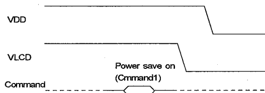
Fig.10 Power supply off timing Case2
