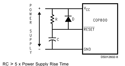
FIGURE 6. Recommended Reset Circuit
