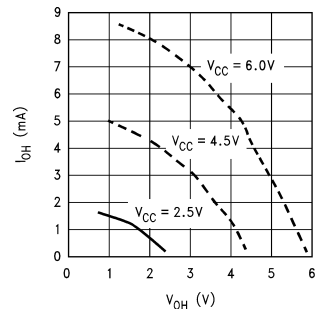
Port L/C/G Push-Pull Source Current
