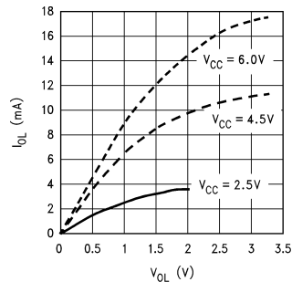
Port L/C/G Push-Pull Sink Current
