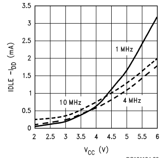
Idle — I_{DD} (Crystal Clock Option)
