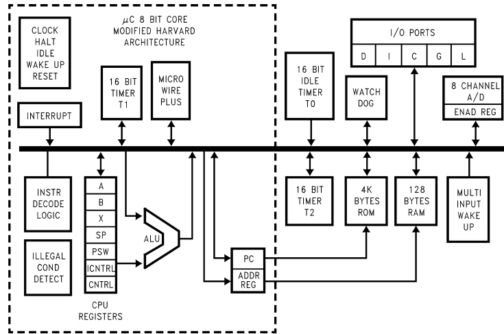
FIGURE 1. Block Diagram
