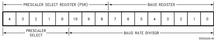
FIGURE 25. USART BAUD Clock Divisor Registers
