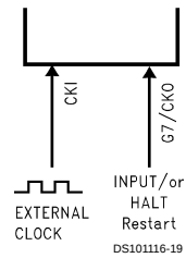
FIGURE 14. External Oscillator
