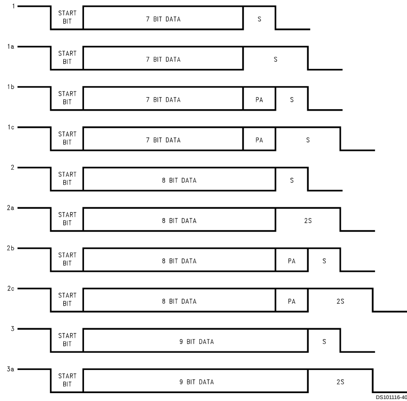
FIGURE 23. Framing Formats
