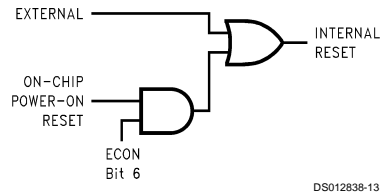
FIGURE 8. Reset Logic
