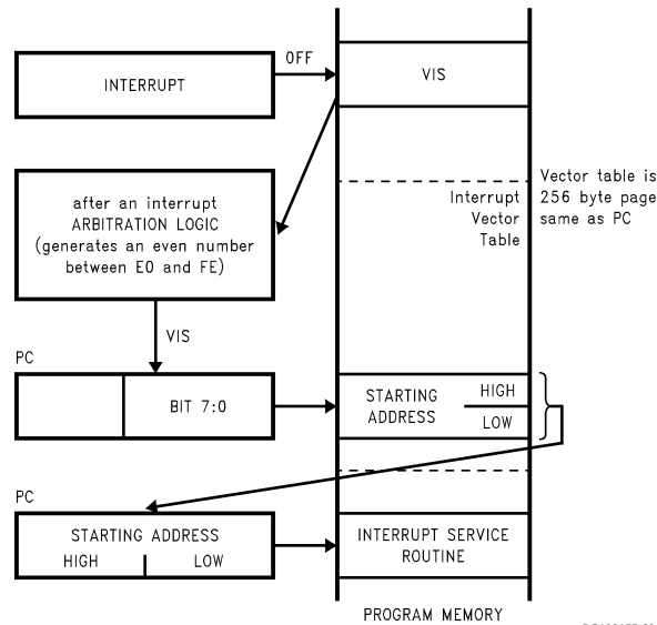
FIGURE 27. VIS Operation
