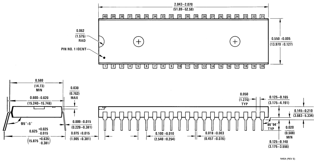
Molded Dual-In-Line Package (N) Order Number COP8SGx740Nx NS Package Number N40A
