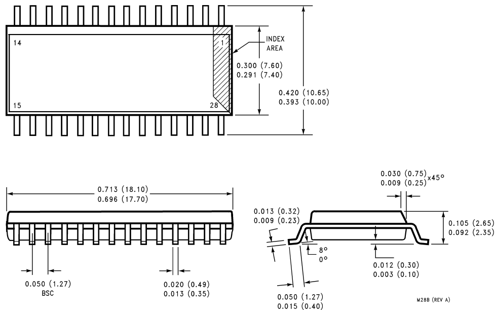
Molded SO Wide Body Package (WM) Order Number COP8SGx728Mx, NS Package Number M28B
