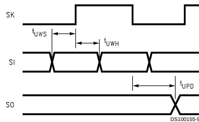
FIGURE 4. MICROWIRE/PLUS Timing
