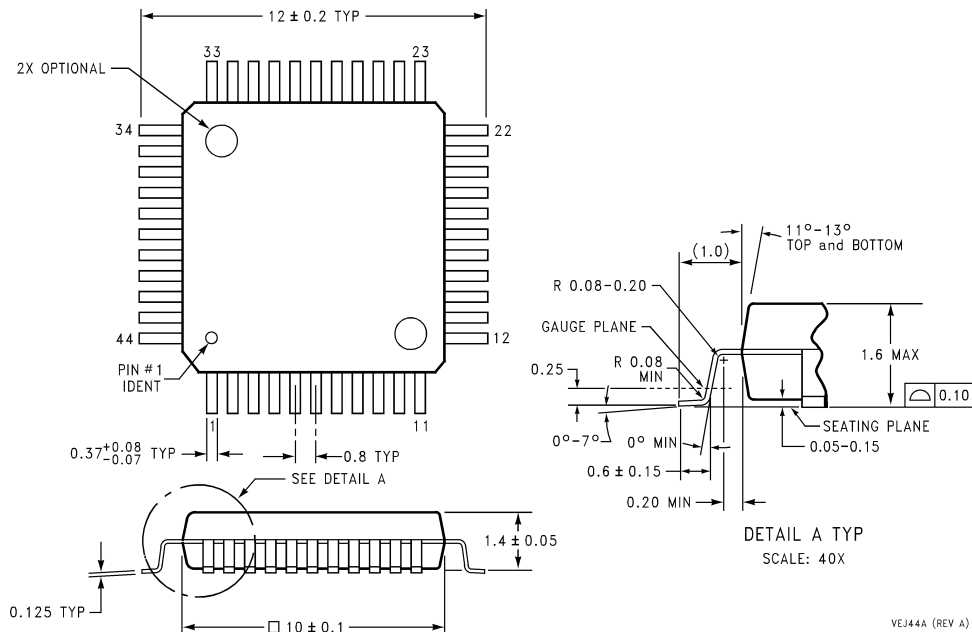
Plastic Quad Flat Package (VEJ) Order Number COP8SGx744VEJx NS Package Number VEJ44A
