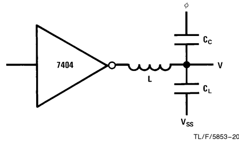
FIGURE 5. Clock Coupling
