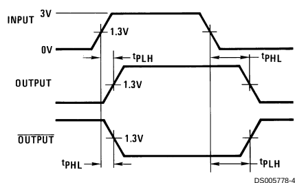
FIGURE 2. Propagation Delays
