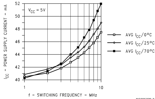
DS26LS31CN Unloaded I_C vs Frequency vs T_A
