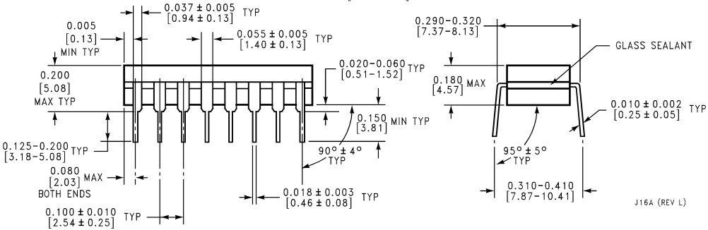
16 Lead Ceramic Dual-in-Line Package (J) Order Number DS26LS31MJ/883 NS Package Number J16A
