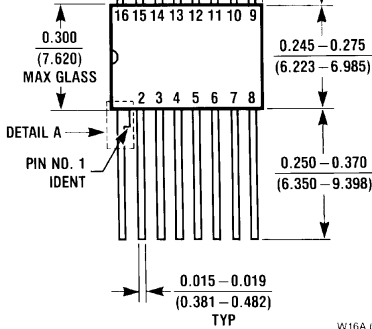
16 Lead Ceramic Flatpak (F) Order Number DS26LS31MW/883 NS Package Number W16A
