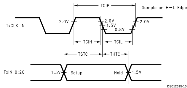
FIGURE 7. DS90CF563 (Transmitter) Setup/Hold and High/Low Times
