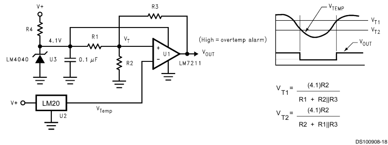
FIGURE 6. Centigrade Thermostat
