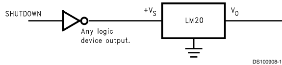
FIGURE 7. Conserving Power Dissipation with Shutdown
