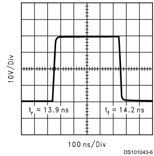
FIGURE 5. LM2438 Pulse Response
