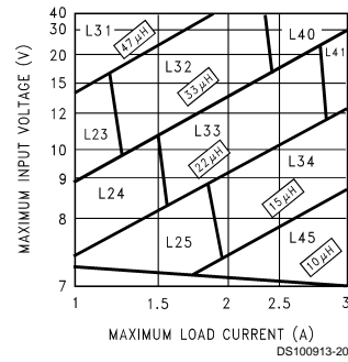
FIGURE 4. LM2673-5.0
