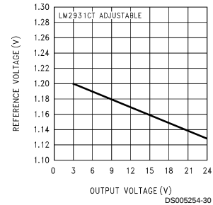
Reference Voltage
