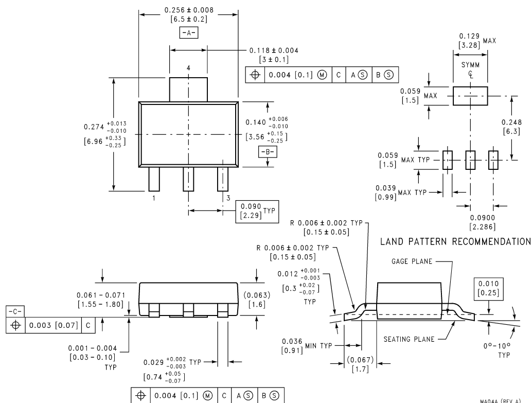
SOT-223 3-Lead Plastic Surface Mount Package Order Number LM2937IMP-5.0, LM2937IMP-8.0, LM2937IMP-10, LM2937IMP-12 or LM2937IMP-15 NS Package Number MA04A
