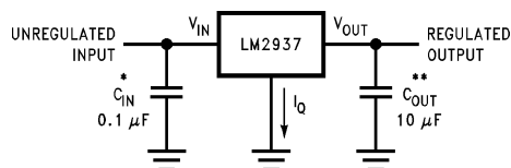
Typical Application
