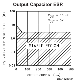
FIGURE 1. ESR Limits
