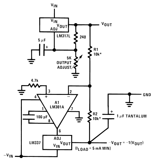
Tracking Regulator
