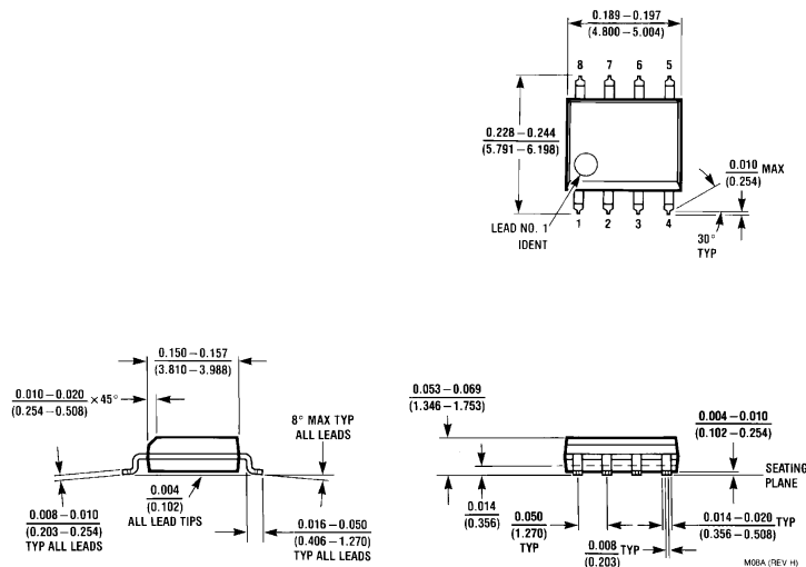
SO-8 Molded Package Order Number LM317LM NS Package Number M08A
