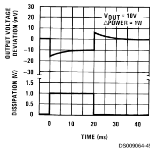
Thermal Regulation
