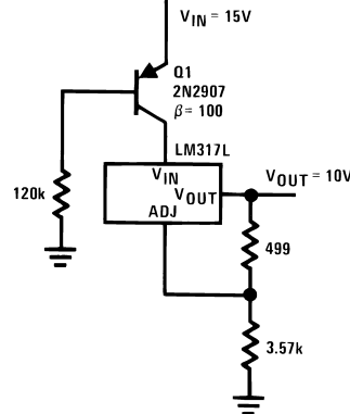
Regulator With 15 mA Short Circuit Current
