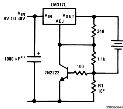
Current Limited 6V Charger
