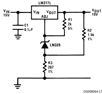
High Stability 10V Regulator
