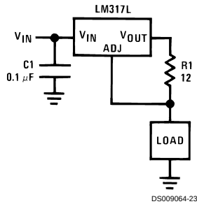
100 mA Current Regulator
