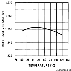
Reference Voltage Temperature Stability
