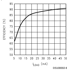
P_{\eta} vs I_{\text{load}} (Step-Up)
