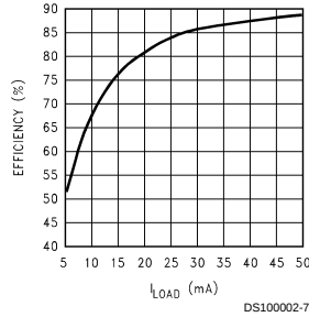
P η vs I load (Step-Down)
