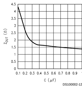
B. Step-Down Mode FIGURE 1. Z_{\text{out}} vs. C
