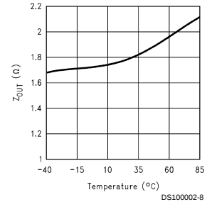
Output Source Impedance vs Temperature (Step-Down)
