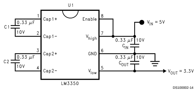
FIGURE 3. Step-Down Converter
