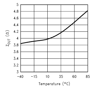
Output Source Impedance vs Temperature (Step-Up)
