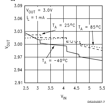
V_{\text{OUT}} vs. V_{\text{IN}}
