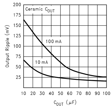
V_{OUT} Ripple vs. C_{OUT}
