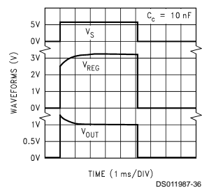
Response Time for 3.3V Version ( C_c = 10 \text{ nF} )
