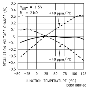
Normalized Temperature Drift
