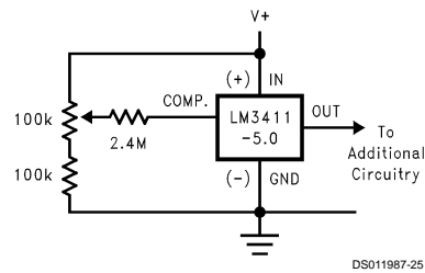
FIGURE 13. \pm 50 mV External Trim
