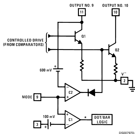
Block Diagram of Mode Pin Description
