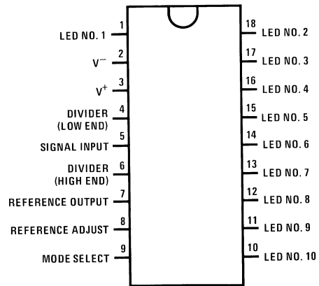
Dual-in-Line Package
