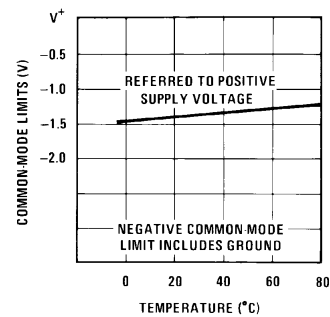
Common-Mode Limits
