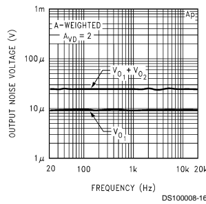
Noise Floor
