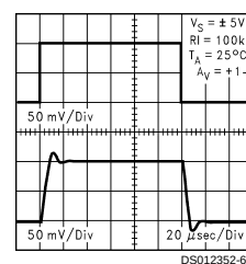
Non-Inverting Small Signal Pulse Response at 10V
