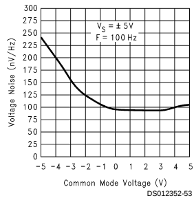
Voltage Noise vs Common Mode Voltage @ 10V
