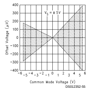
Offset Voltage vs Common Mode Voltage @ 10V
