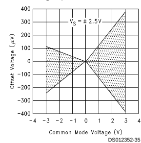
Offset Voltage vs Common Mode Voltage @ 5V
