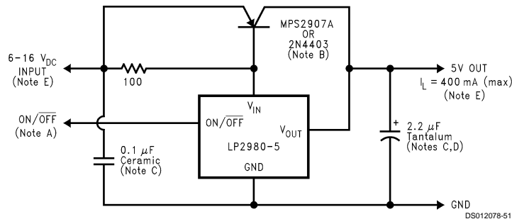
FIGURE 5. 5V/400mA Regulator
