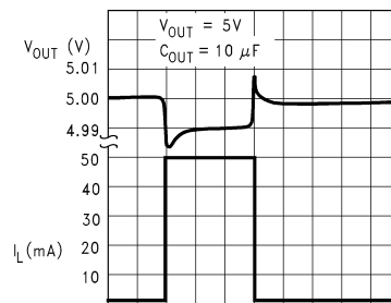
Load Transient Response
