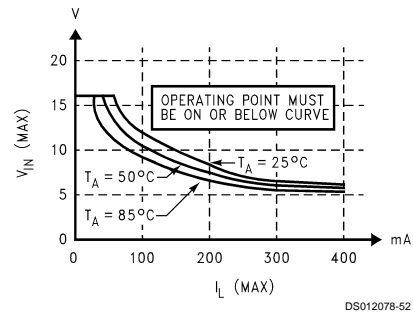
FIGURE 6. Safe Operation Boundary Curves for Figure 5
