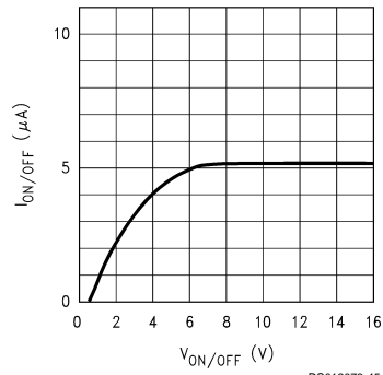
ON/OFF Pin Current vs V_{ON/OFF}
