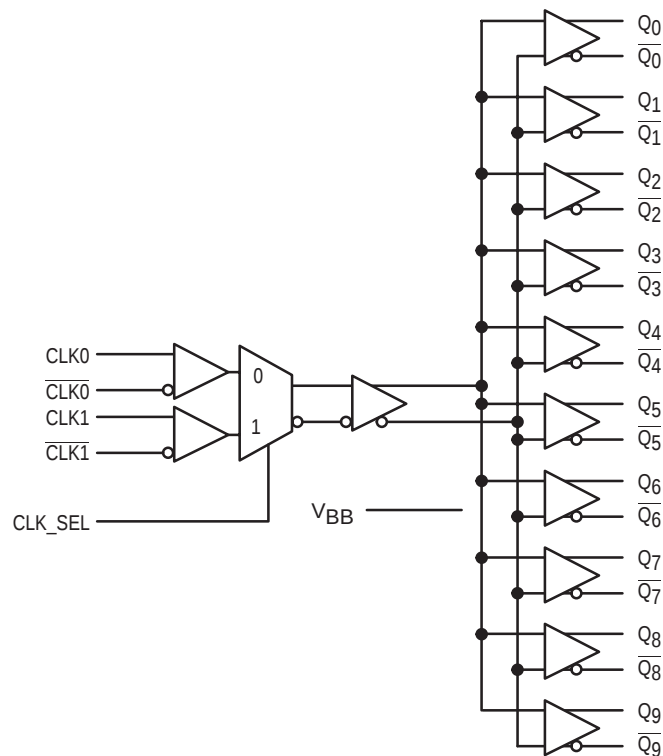
Figure 2. Logic Symbol
