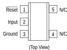
N SUFFIX PLASTIC PACKAGE CASE 1212 (SOT-23)
