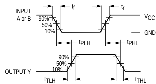
Figure 3. Switching Waveforms
