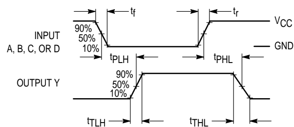
Figure 1. Switching Waveforms
