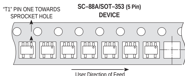
Figure 11. Reel Configuration
