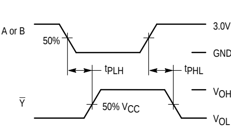
Figure 3. Switching Waveforms
