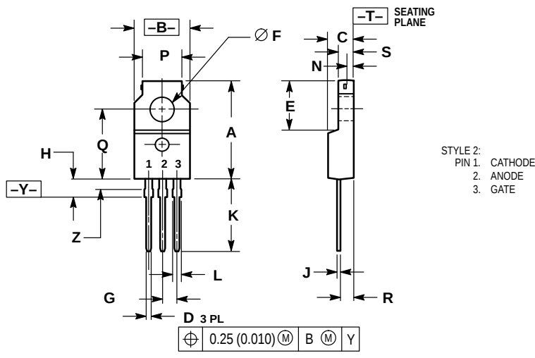
CASE 221C-02 ISSUE B
