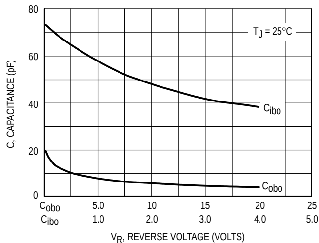
Figure 6. Capacitance
