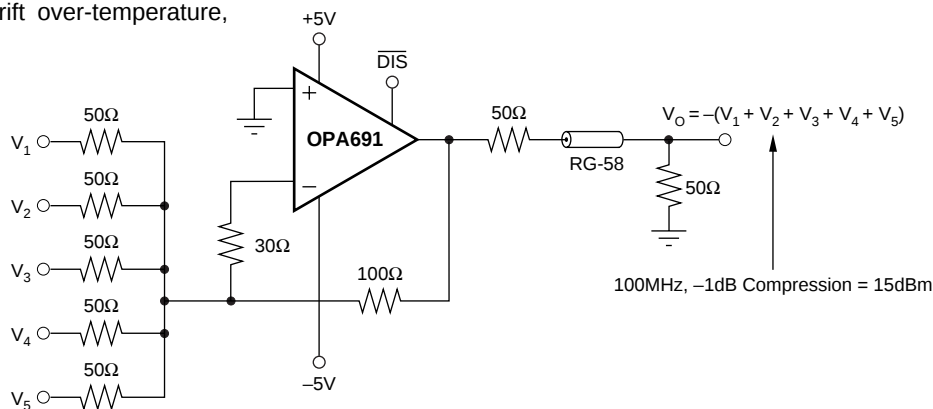
200MHz RF Summing Amplifier
